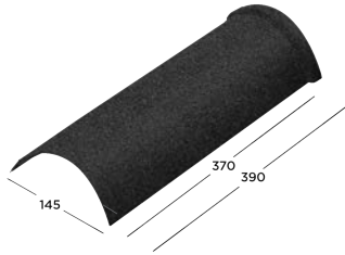
BARREL TRIM
