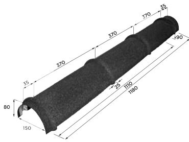
BARREL THREE ELEMENTS
