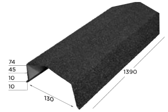
RECTANGULAR RIDGE
