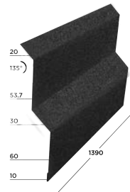
WALL FLASHING
