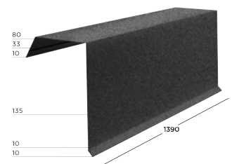
BOX BARGE
