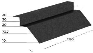
EAVES FLASHING
